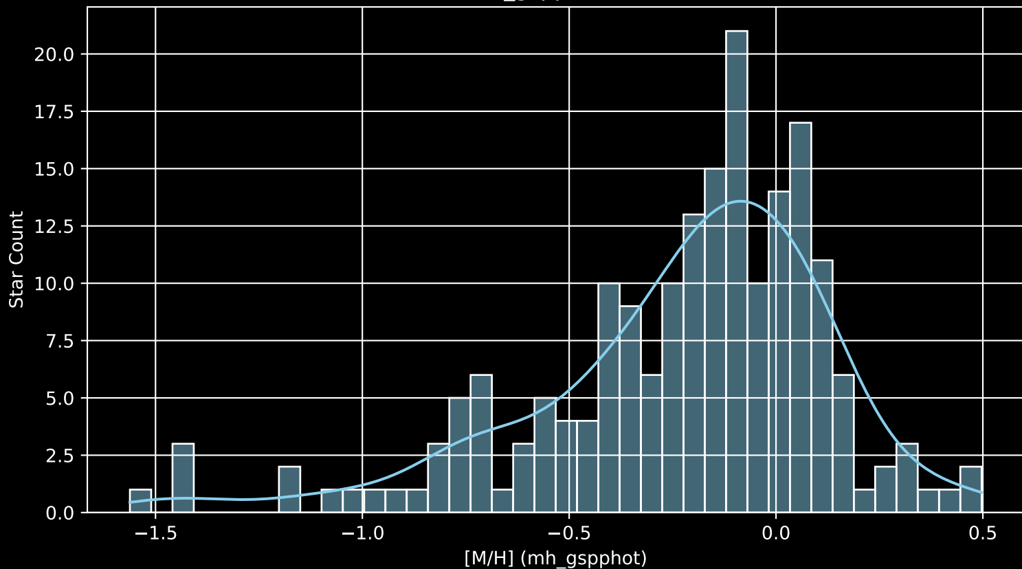
APOGEE DR17 Field: [K2_C4_167-24_btx [M/H] (mh_gspphot) (n= 194)
