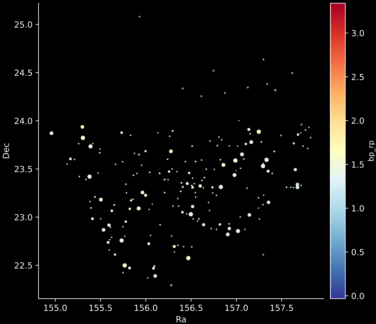
APOGEE DR17 Field: [K2_C4_167-24_btx] Stars: 196
