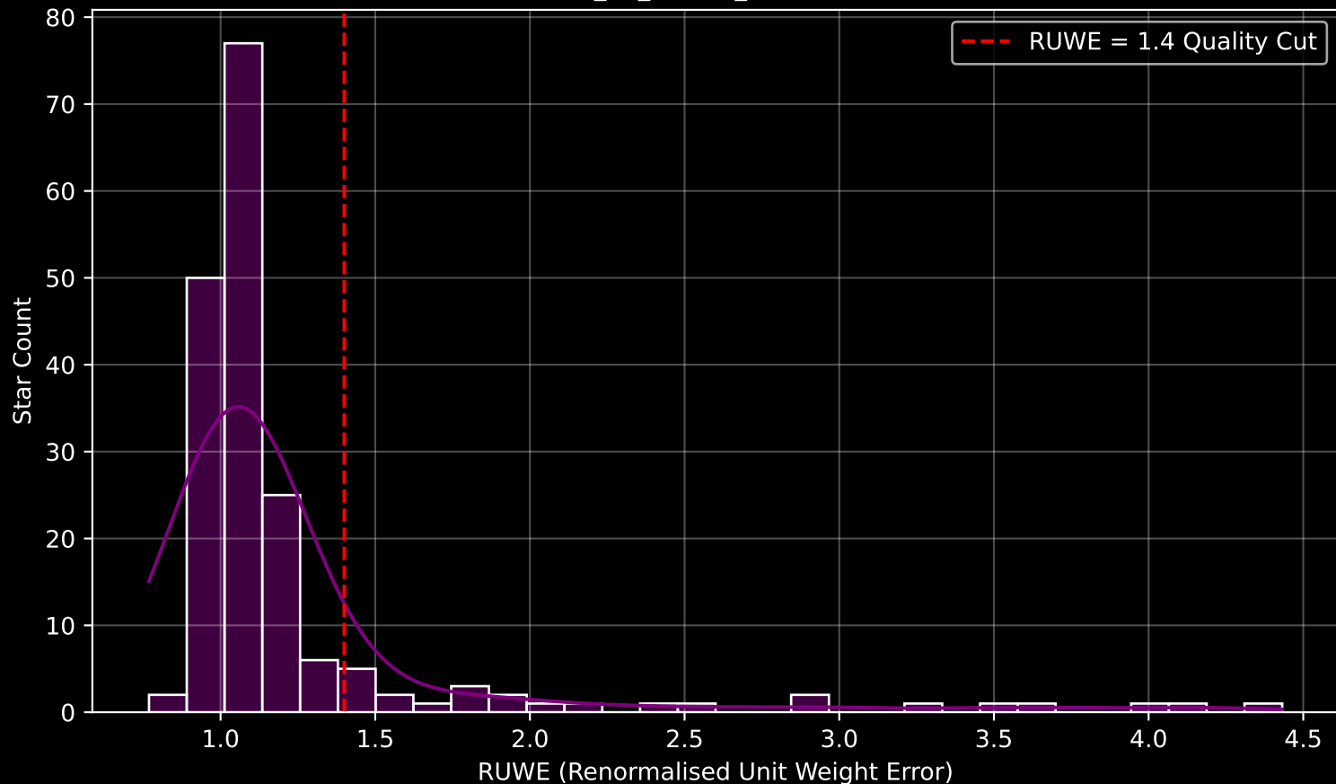
GAPOGEE DR17 Field [K2_C4_167-24_btx] RUWE Distribution (n= 185)
