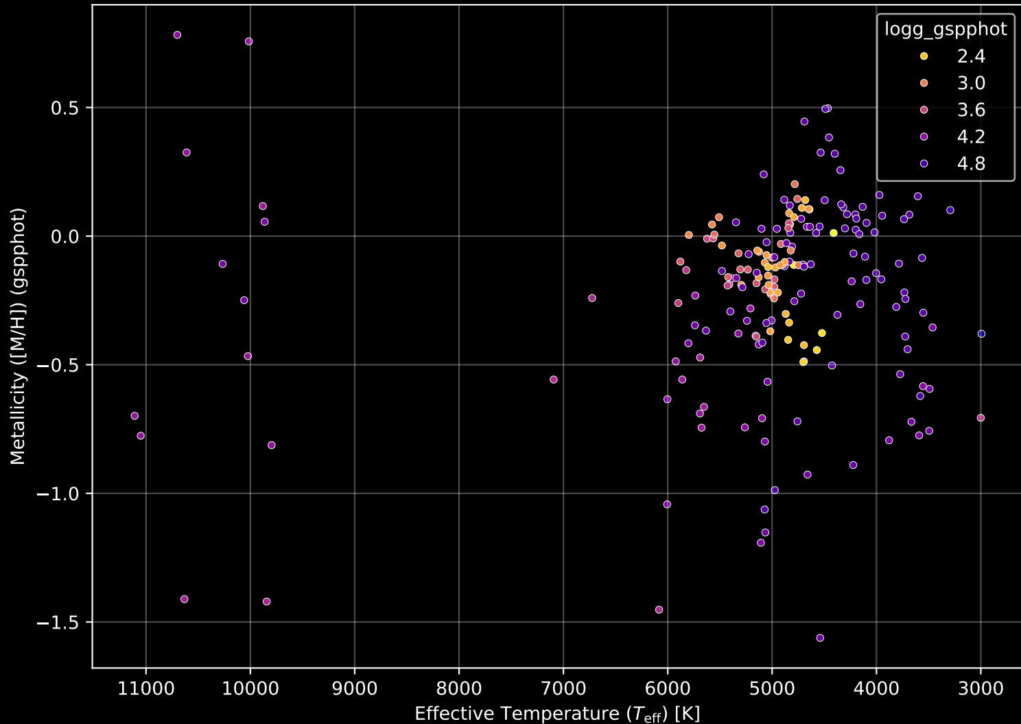
APOGEE DR17 Field: [K2_C4_167-24_btx] Stellar Population Parameters (n= 196)
