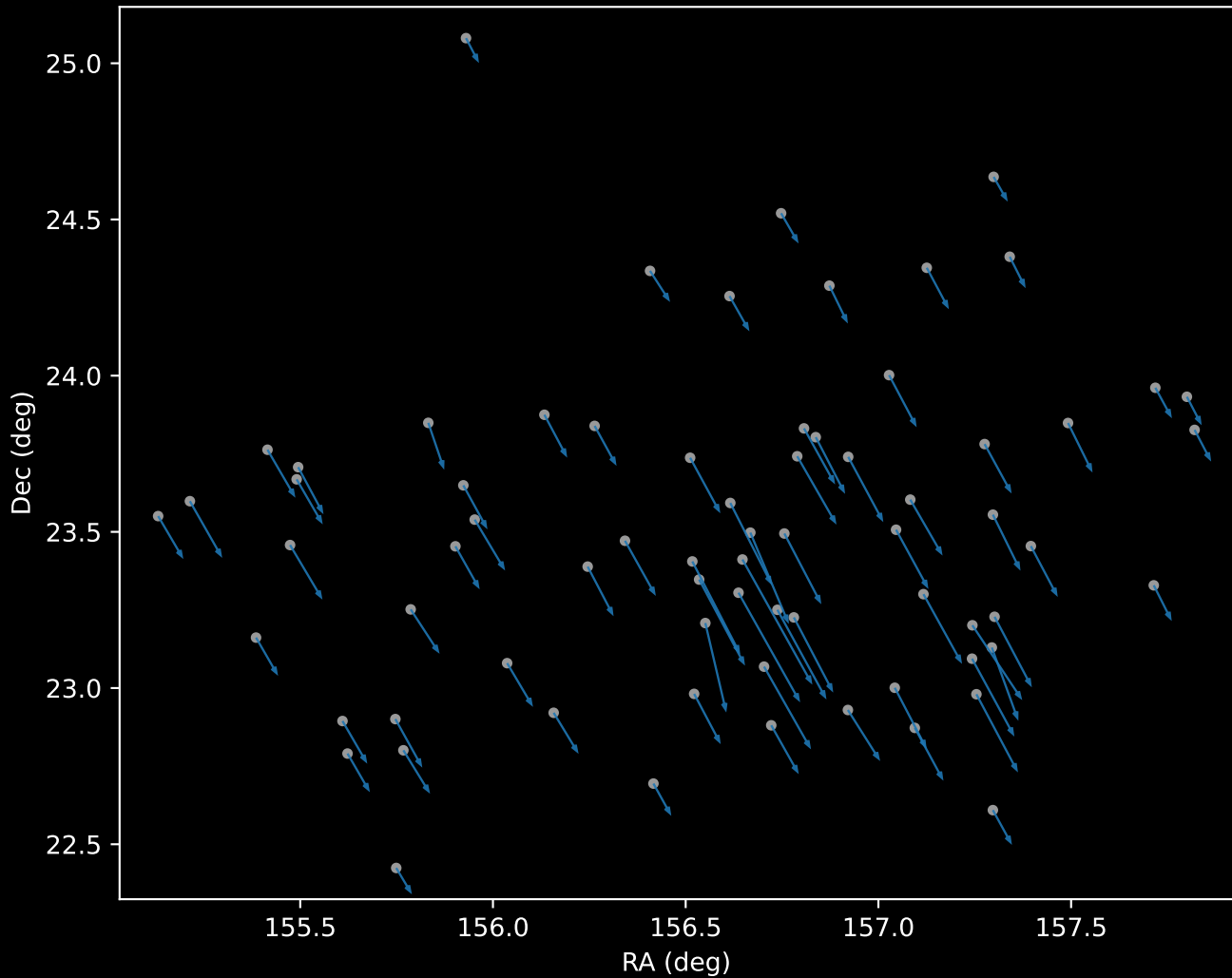
APOGEE DR17 Cluster 0 Proper Motion Vectors (n=71)
