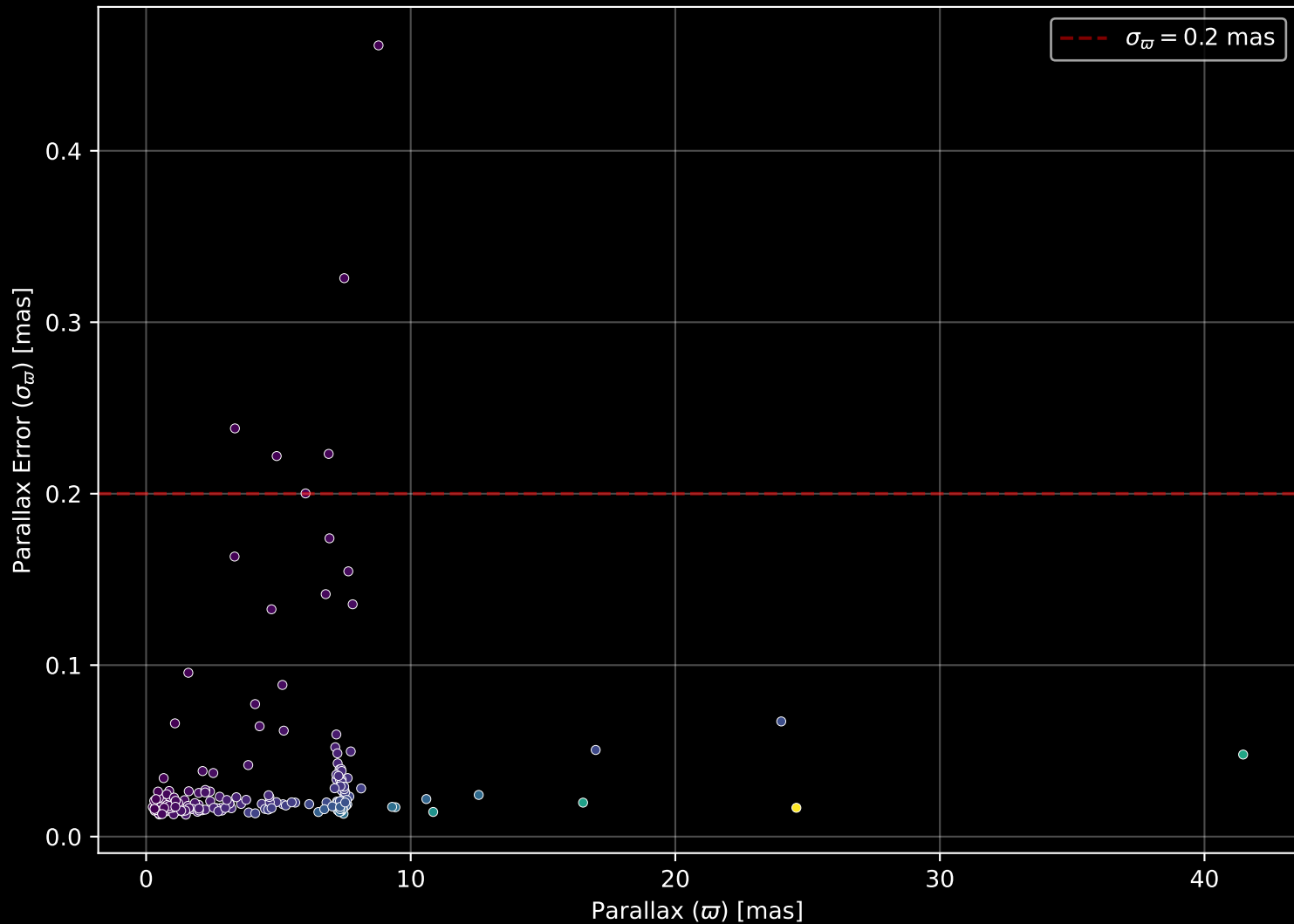
APOGEE DR17 Field: [K2_C4_167-24_btx] Parallax Quality (n= 196)
