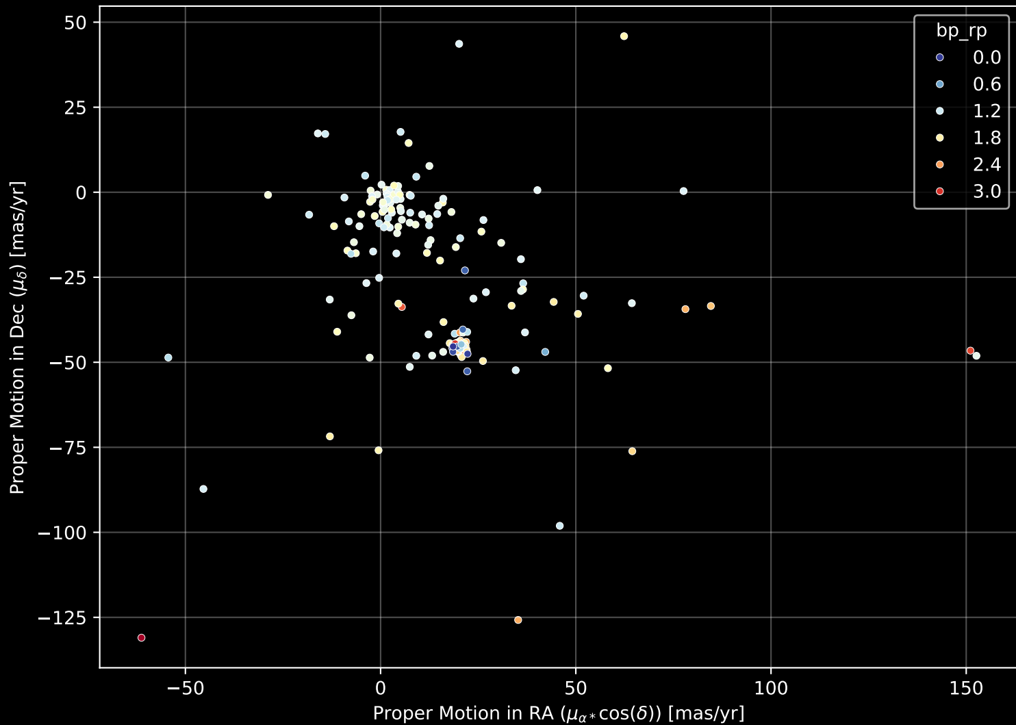
APOGEE DR17 Field: [K2_C4_167-24_btx] Proper Motion Diagram (n= 196)
