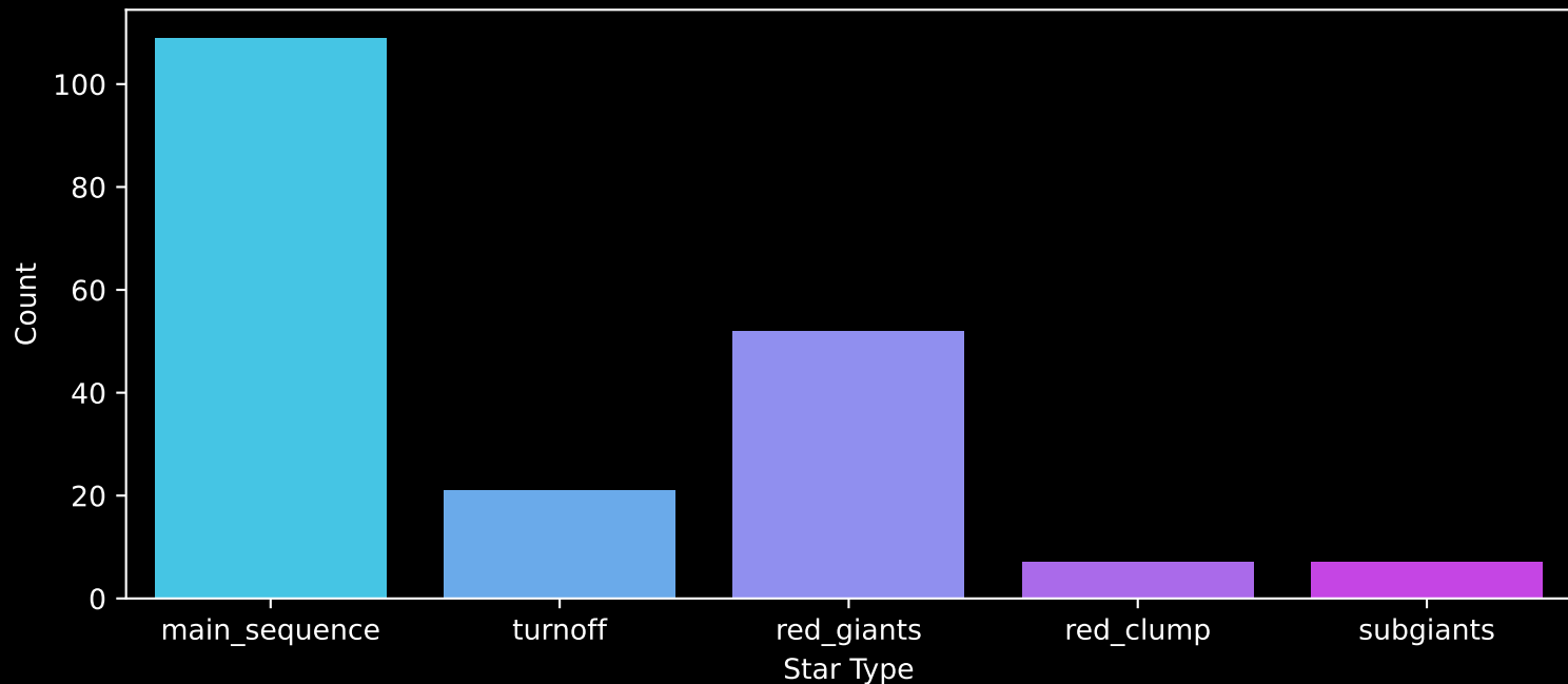
APOGEE DR17 Field: [K2_C4_167-24_btx] Count plot of Star Type
